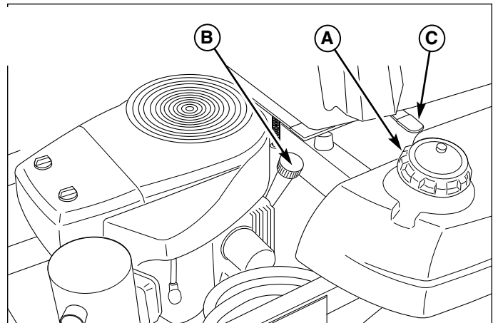
Figure 2. Pre-start Checks
