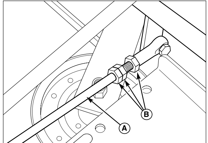
Figure 28. Neutral Adjustment (LH side shown with battery removed) A. Adjustment Linkage Rod B. Nuts
