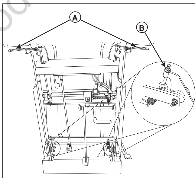
Figure 38. Reverse Speed Control Levers Comfort Adjustment
