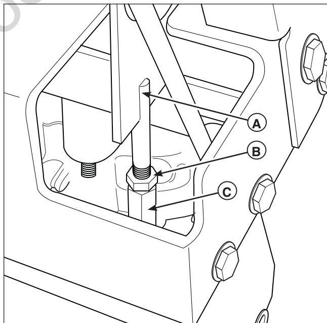
Figure 25. Adjusting the Speed of the Faster Wheel (RH side shown)
