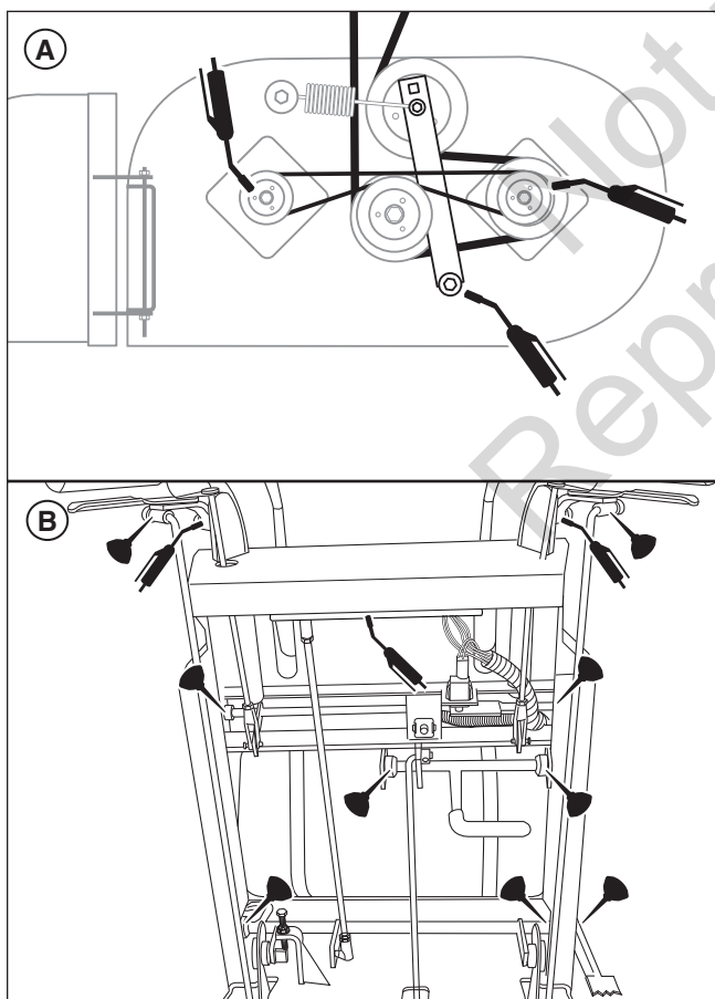
Figure 14. Lubrication Points
