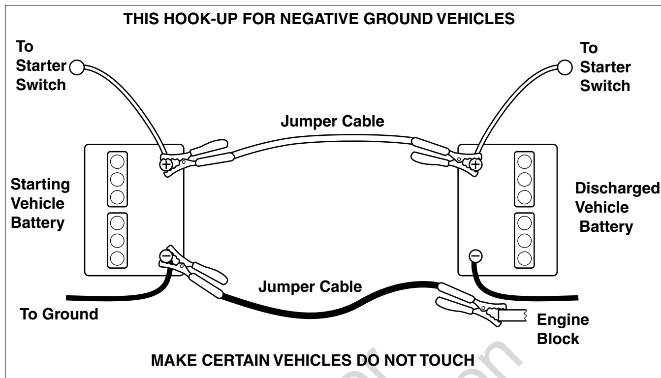
Figure 41. Jump Starting
