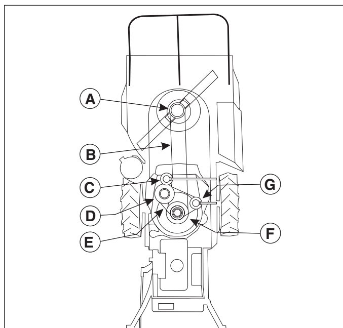
Figure 24 - Belt Alignment
