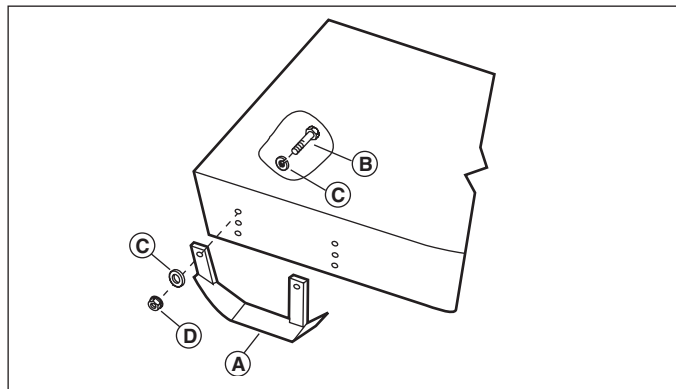
Figure 9 - Adjusting Height
