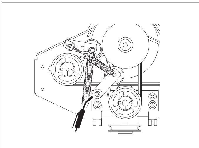
Figure 17. Gearbox Drive Idler Pivot
