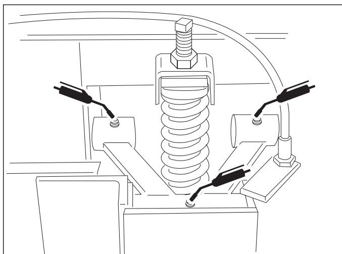
Figure 19. Rear Suspension Lubrication (Both upper & lower a-arms)
