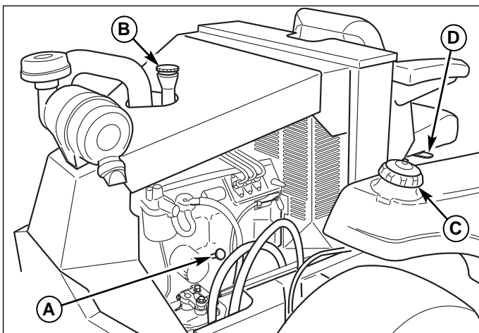
Figure 4. Pre-Start Checks (Diesel model shown, gas model in similar locations) A. Crankcase Dip Stick B. Oil Fill Cap C. Fuel Tank Cap (both sides) D. Seat Adjustment Lever
