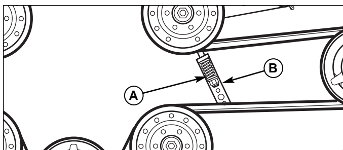
Figure 49. Mower PTO Belt
