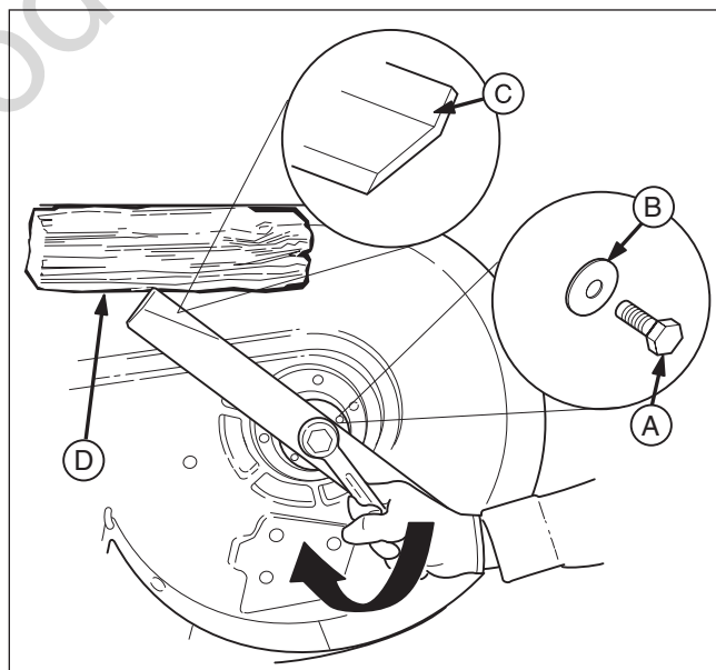
Figure 34. Tightening the Mower Blade for Installation
