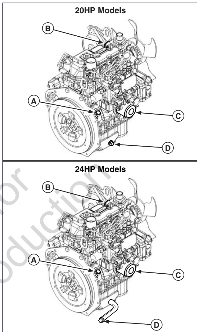
Figure 15. Engine Oil Fill
