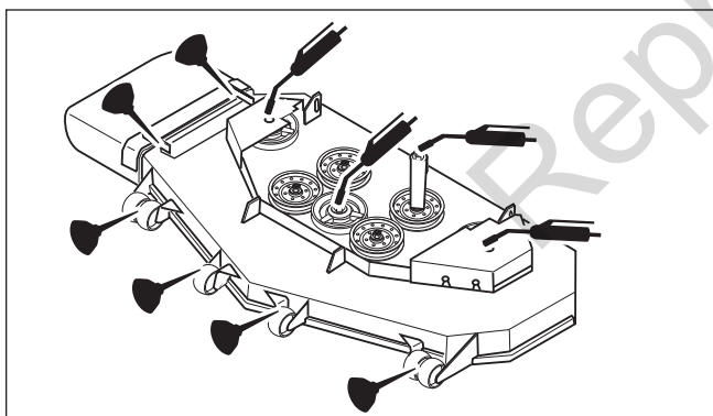
Figure 20. Deck Lubrication
