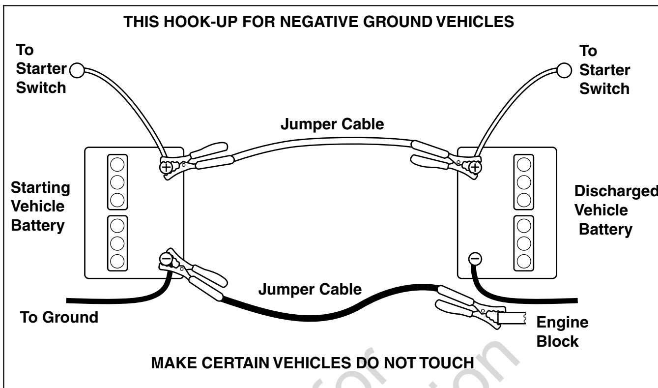
Figure 65. Jump Starting
