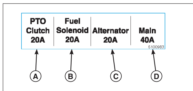
Figure 35. Fuse Location Decal
